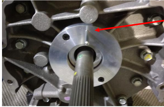
FIGURE H MAGNUM BEARING RETAINER
